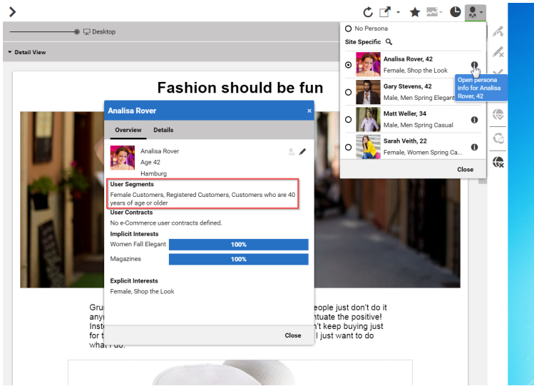
Figure 9.9. Test Customer Persona with Commerce Customer Segments
