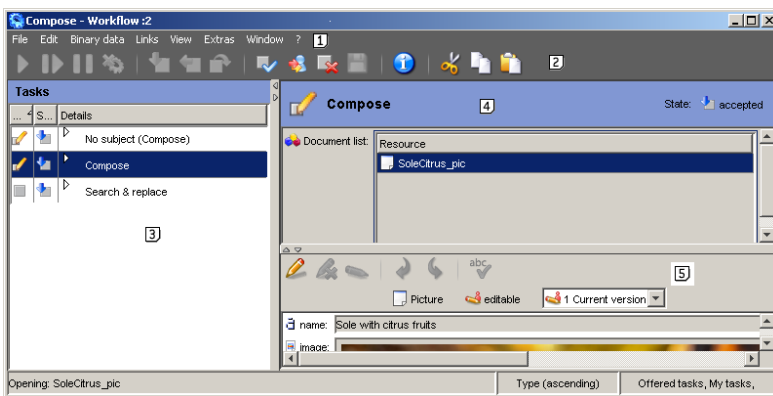
Figure 2.3. Workflow window
