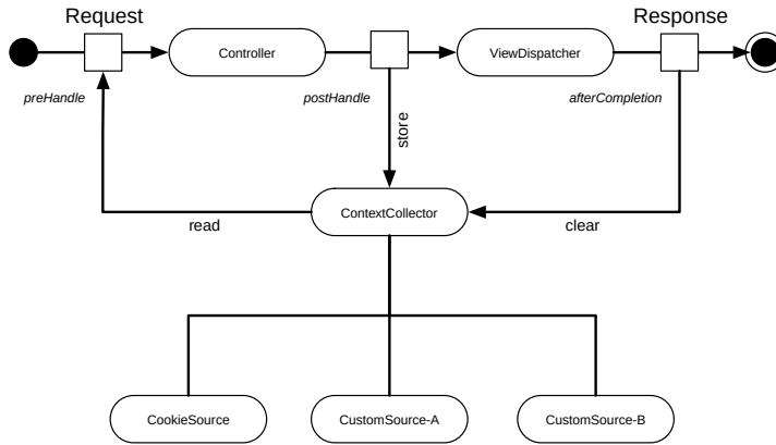
Figure 4.4. ContextCollector position
