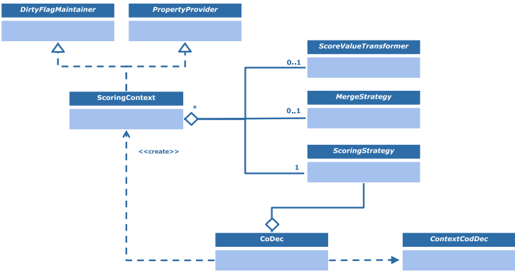
Figure 4.9. Scoring classes
