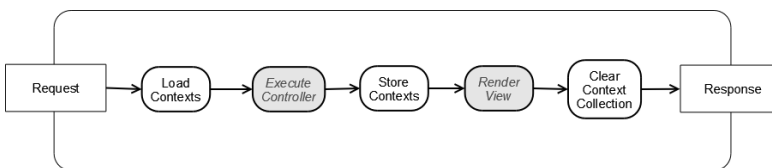
Figure 4.3. ContextObject usage
