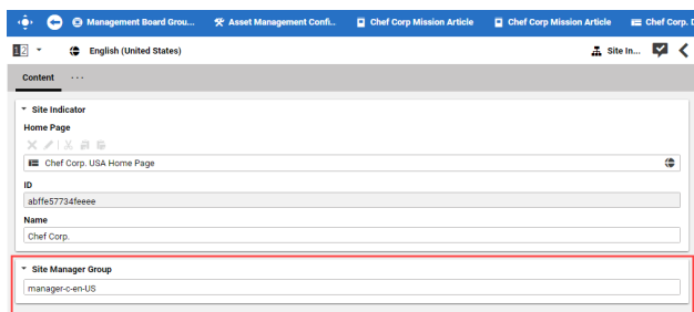
Figure 5.29. Site Indicator: Setting site manager group
