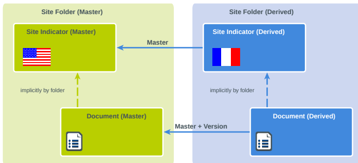
Figure 5.26. Multi-Site Interdependence
