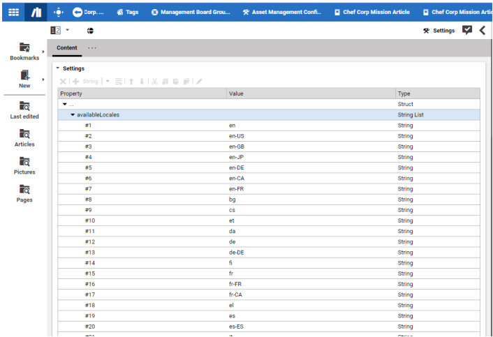
Figure 5.27. Locales Administration in CoreMedia Studio
