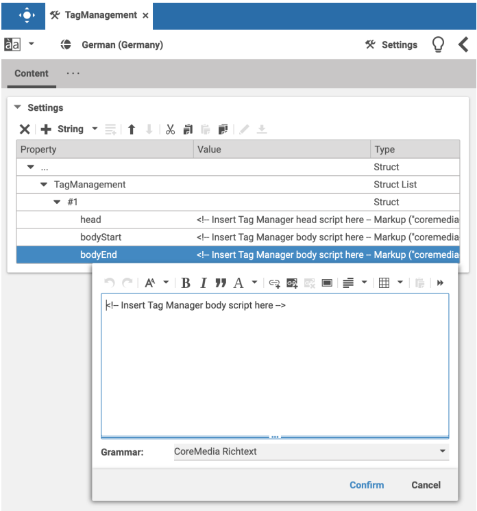
Figure 5.25. Tag Management Configuration
