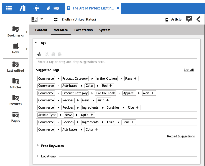
Figure 5.6. Taxonomy Property Editor
