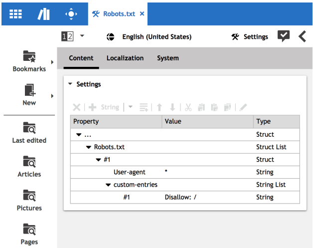
Figure 5.18. Channel settings with configuration for Robots.txt as a linked setting on a root page
