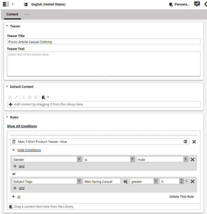
Figure 6.23. Conditions in Personalized Content and Customer Segment documents
