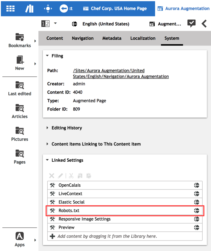
Figure 5.17. Robots.txt settings
