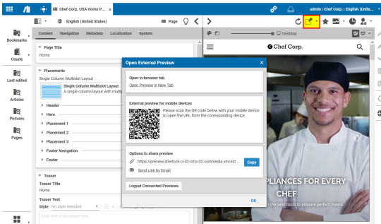
Figure 6.11. External Preview
