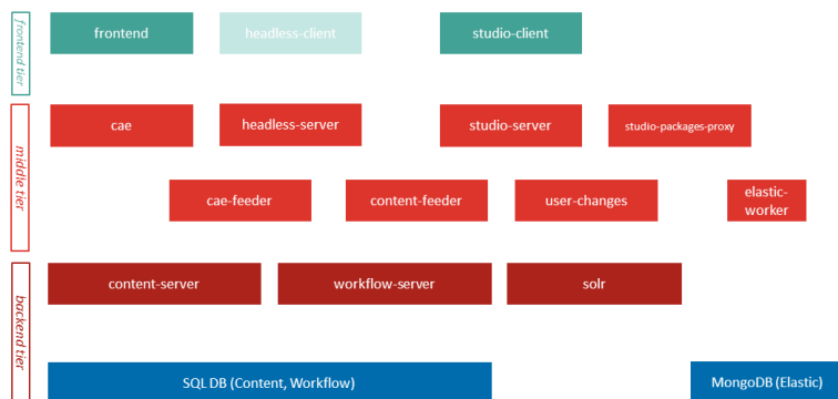
Figure 4.1. CoreMedia CMS's Four-Tier Architecture
