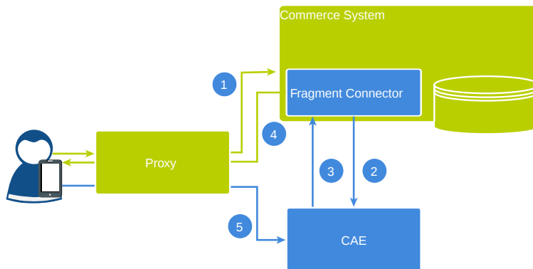
Figure 8.7. Cross Site Scripting with fragments
