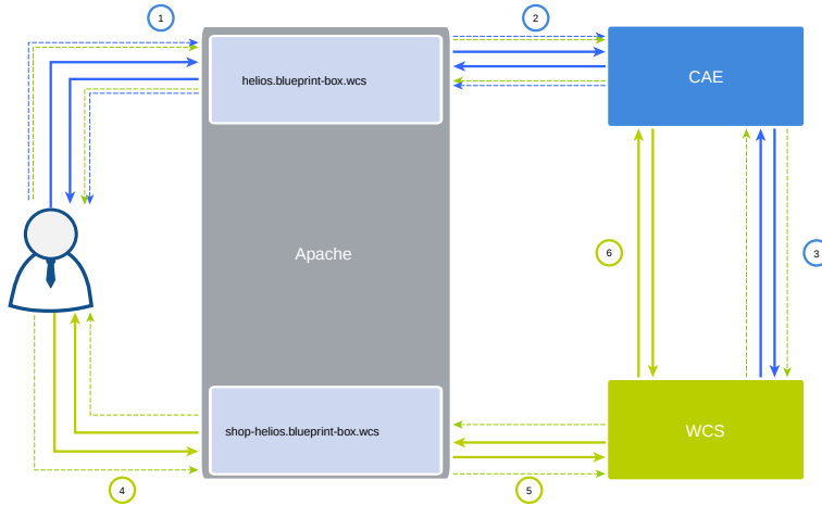
Figure 9.2. Content-led integration scenario with cookies
