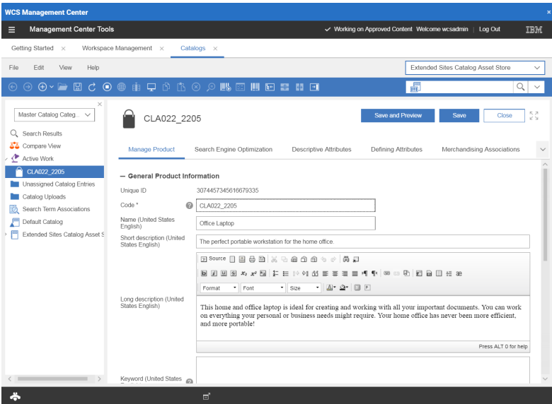
Figure 10.9. Management Center in Studio
