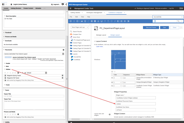
Figure 8.4. Connection via placement name
