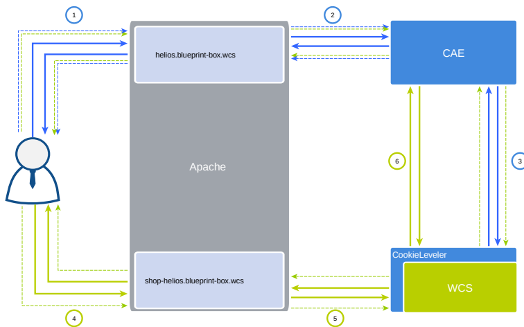
Figure 9.3. Content-led integration scenario
