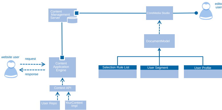
Figure 4.1. Adaptive Personalization overview
