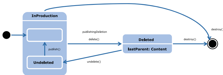
Figure 5.4. Statechart: Deleting
