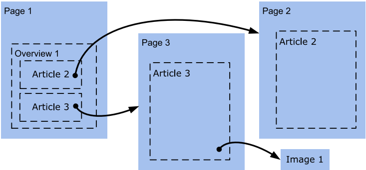
Figure 4.3. Entity Model
