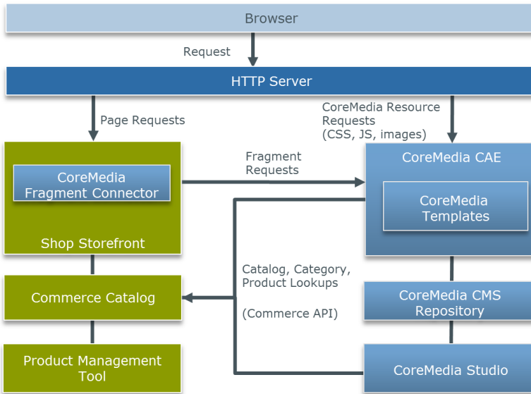
Figure 6.1. Commerce-led Architecture Overview
