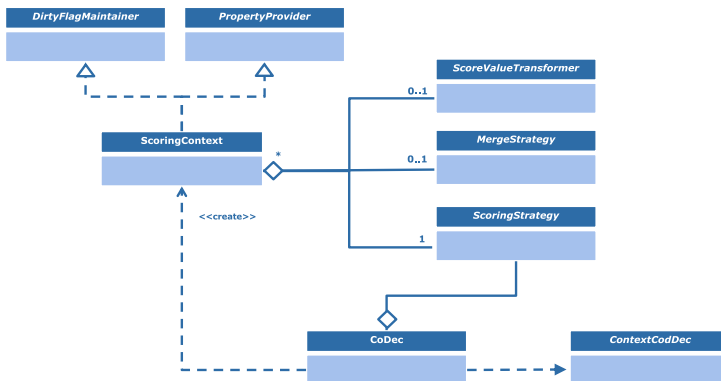
Figure 4.9. Scoring classes
