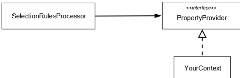
Figure 4.6. PropertyProvider Interface
