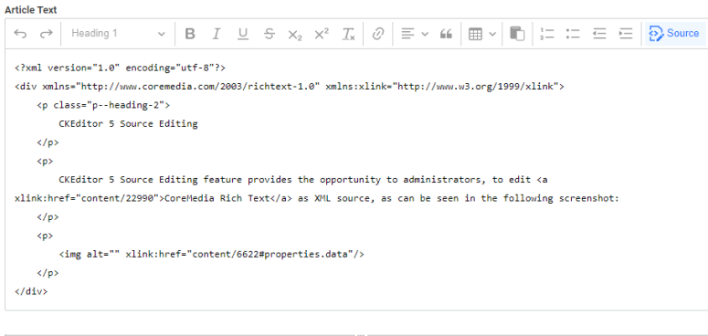
Figure 10.2. CKEditor 5 Source Editing Feature
