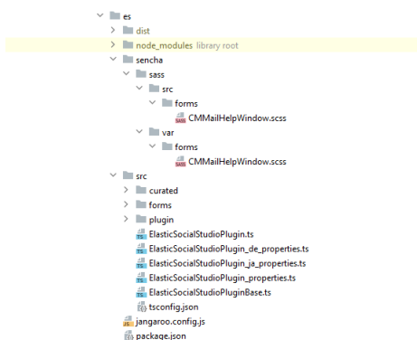
Figure 9.2. Plugin structure
