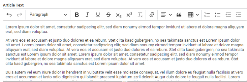
Figure 10.4. CKEditor 5
