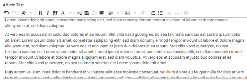
Figure 10.3. CKEditor 4
