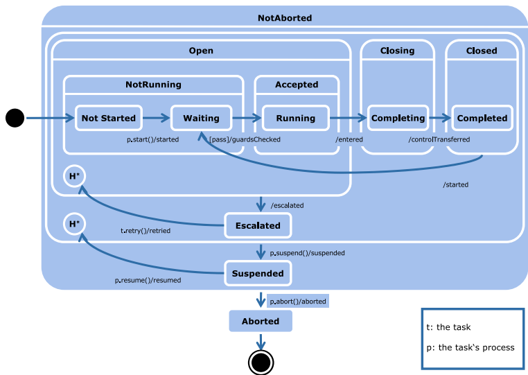
Figure 6.3. States of an automated task
