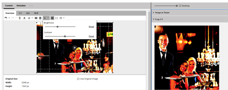
Figure 4.79. Exposure controls
