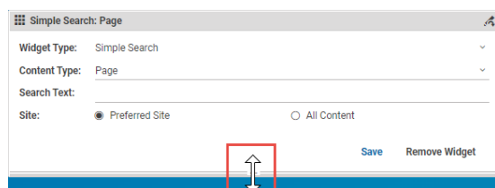
Figure 4.4. Scale widget
