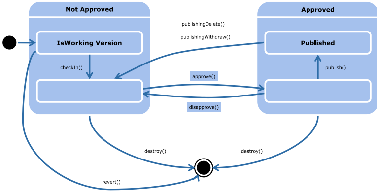
Figure 5.5. Statechart: Version
