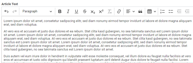
Figure 10.4. CKEditor 5
