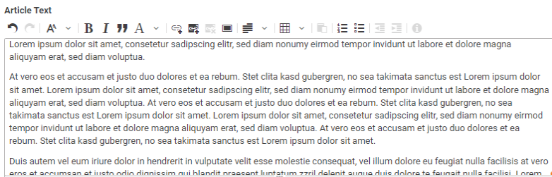
Figure 10.3. CKEditor 4
