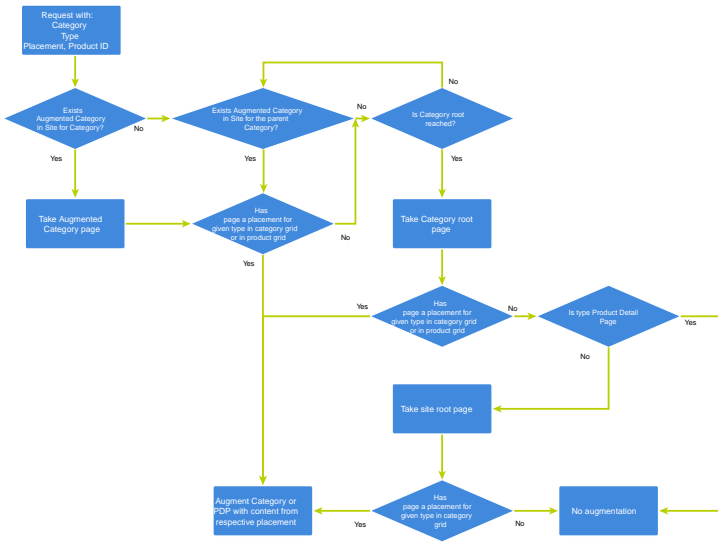
Figure 6.21. Decision diagram
