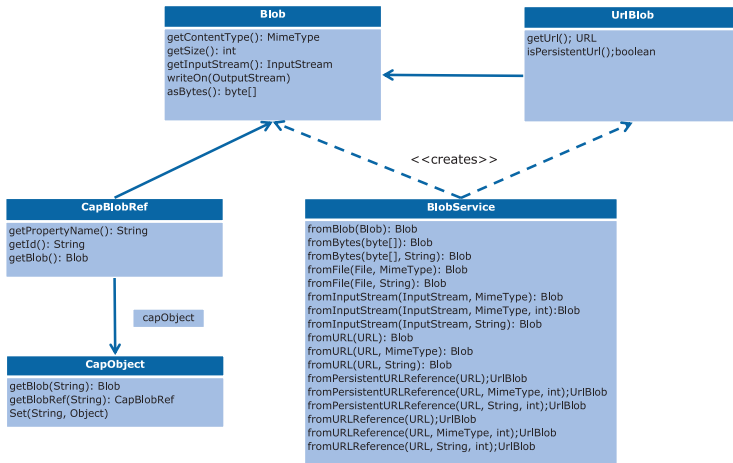
Figure 4.2. Class Diagram: Blobs
