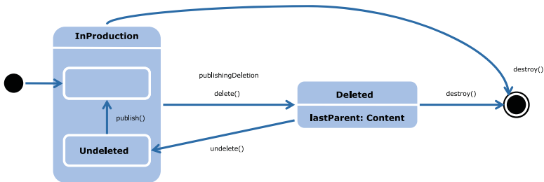
Figure 5.4. Statechart: Deleting
