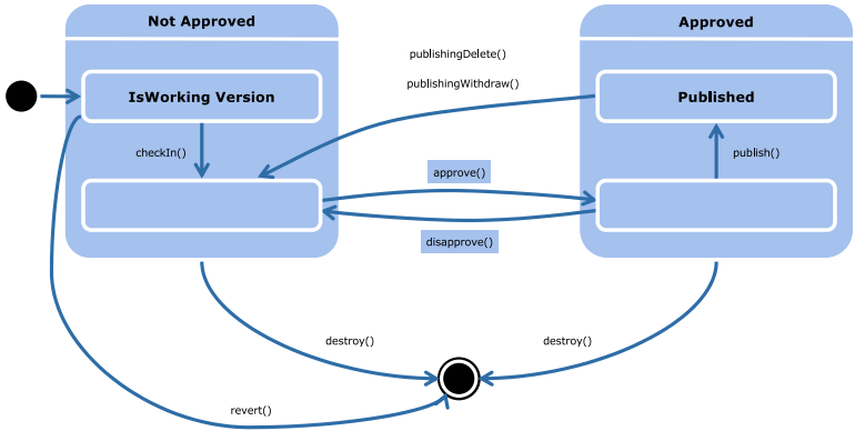
Figure 5.5. Statechart: Version
