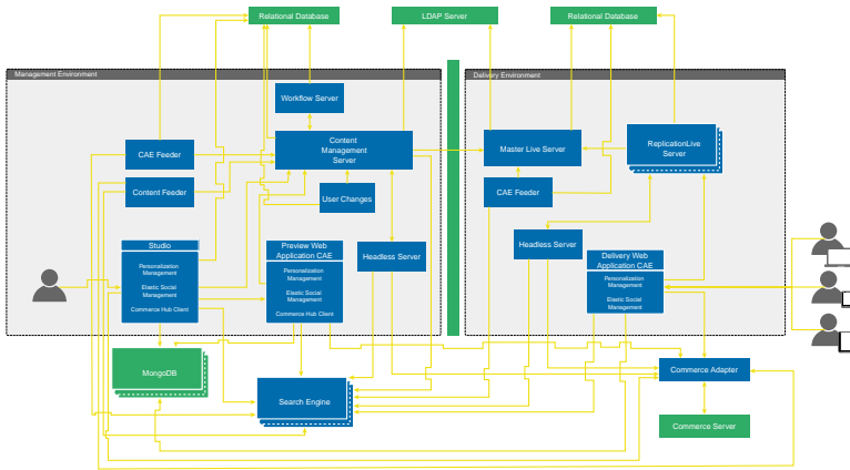
Figure 2.1. System Overview
