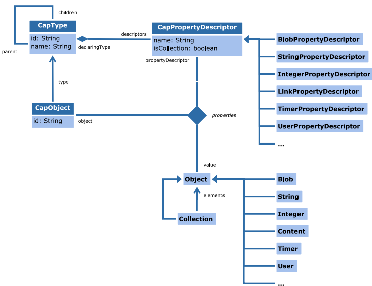
Figure 4.3. Class Diagram: Types
