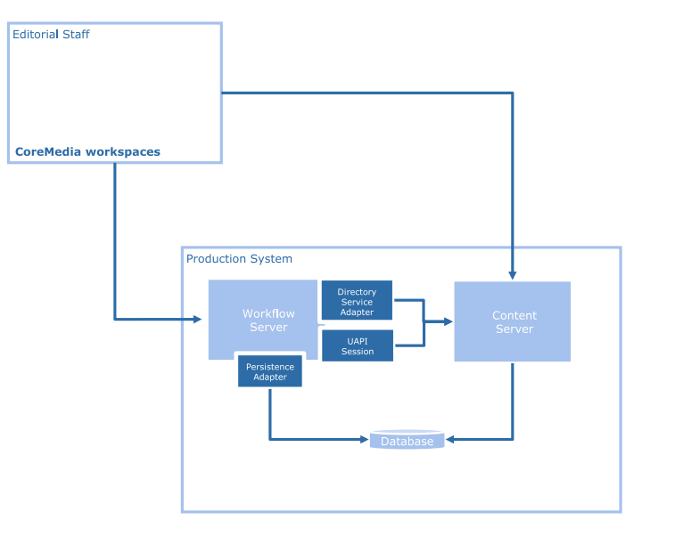
Figure 2.1. CoreMedia architecture with integrated workflow
