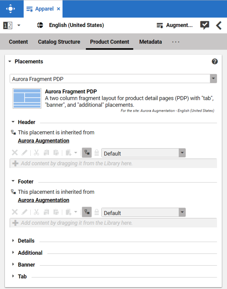
Figure 6.12. Page grid for PDPs in augmented category
