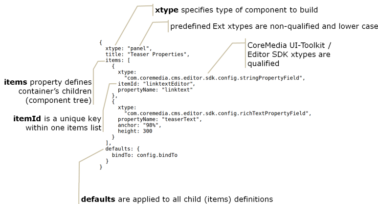
Figure 5.1. Ext JSON
